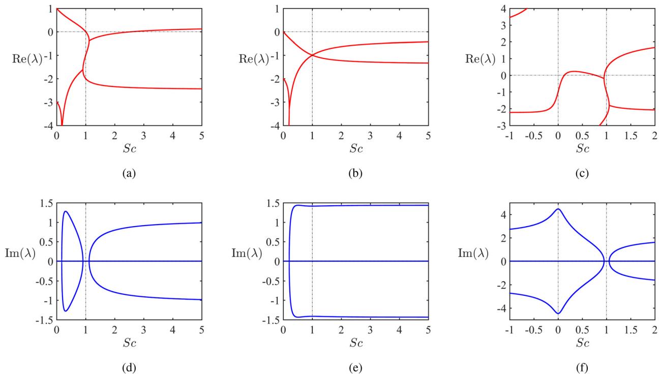
FIG. 4. Growth rates and frequencies for m = 0 , Ek = 1 , Ro = 1 , and (a and d) \gamma_1 = -4 , \gamma_2 = 3 , (b and e) \gamma_1 = -1 , \gamma_2 = 3 , (c and f) \gamma_1 = 20 , \gamma_2 = -22 , demonstrating exchange of monotonic and oscillatory instabilities near Sc = 1 , cf. Fig. 2.
