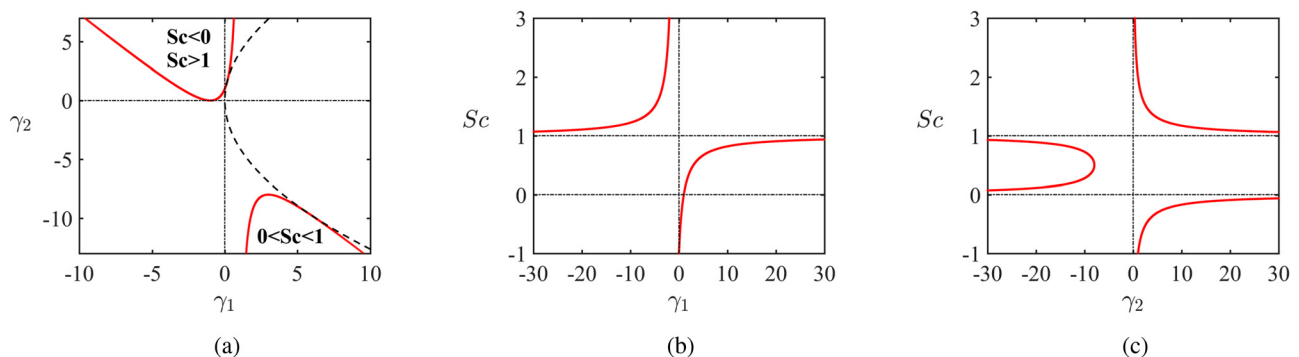
FIG. 3. For Ek=1 , projections of the loci of the codimension-2 points onto (a) (\gamma_1, \gamma_2) plane, (b) (\gamma_1, Sc) plane and (c) (\gamma_2, Sc) plane, given by Eqs. (71) and (72). The dashed curve is the envelope given by Eq. (75).
